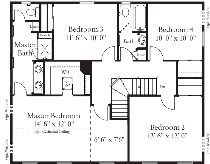
Second Floor Plan with First Floor Laundry
