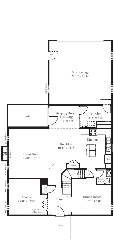
First Floor Plan with Attached Rear Load Garage
